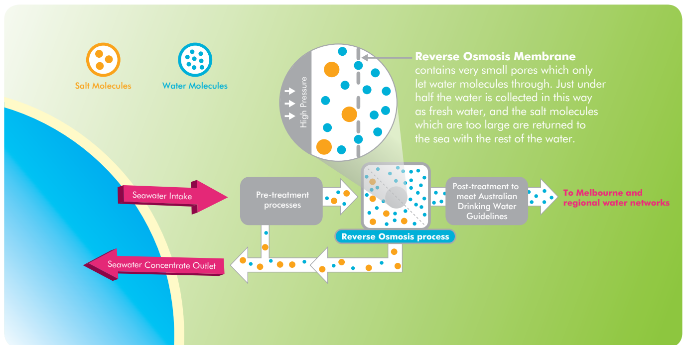
Simple outline of Reverse Osmosis Process
