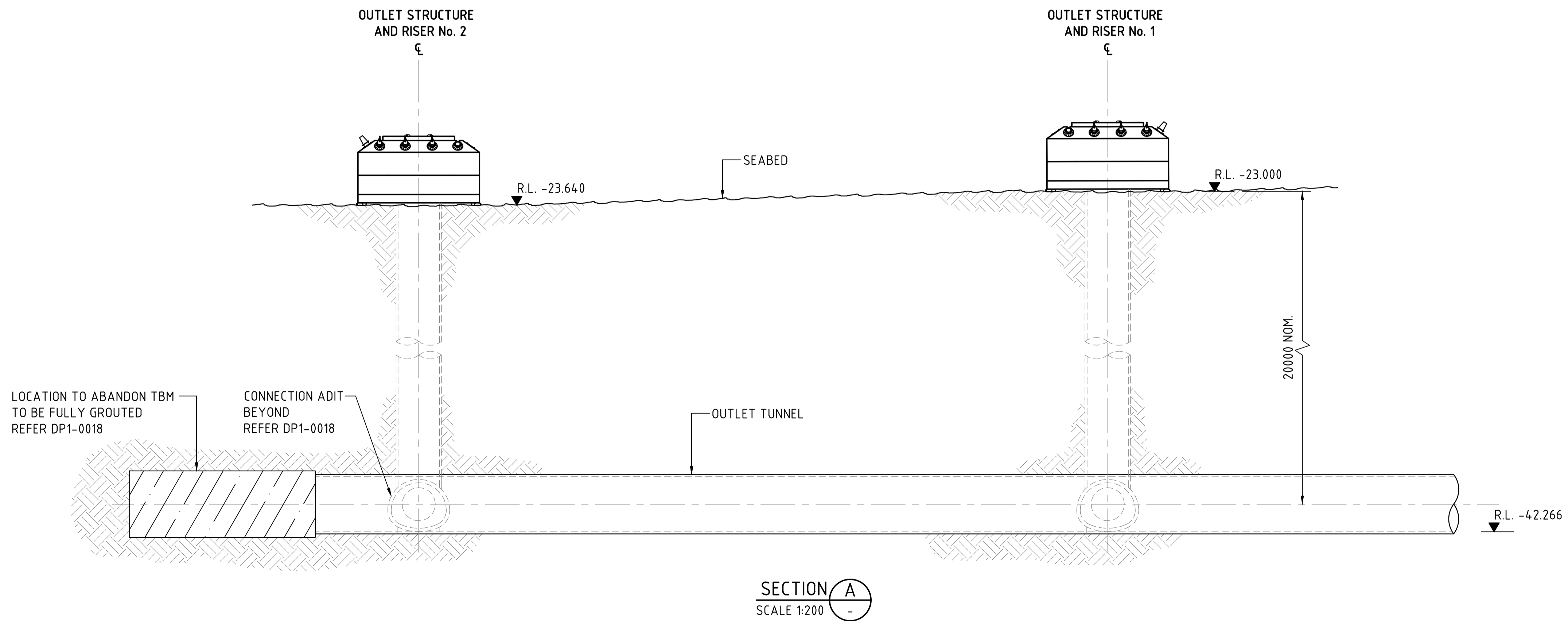
OUTLET STRUCTURE AND RISERS - GENERAL ARRANGEMENT SCALE 1:200
